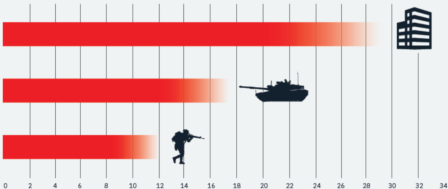
Figure 1: DP-ELRF | MLRF-2B Ranging Performance Using Various Targets (FAR \leq 0.1%)
