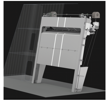
Overhead Foldable Door (four panels)
