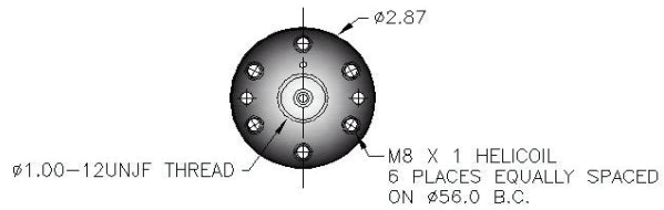
VIEW B-B
