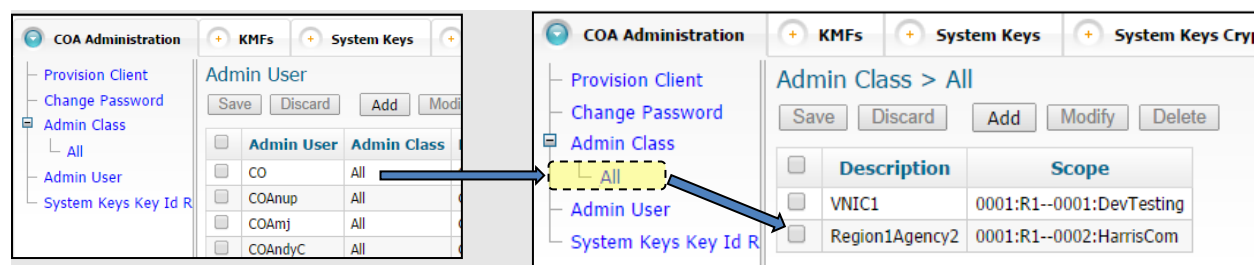
Figure B-6: Admin Class Settings for Crypto Officer in UAS
