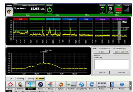
Spectrum analysis
