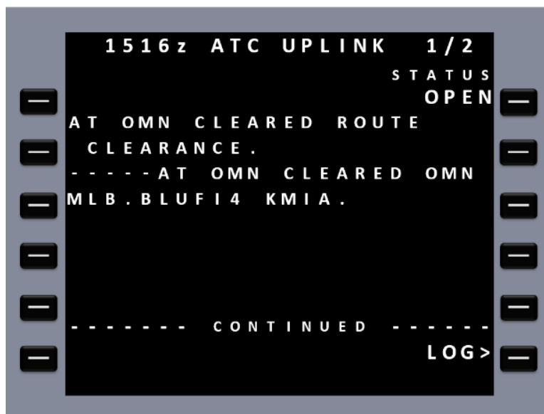
Figure 25. UM83 CPDLC Message Example: AT [position] CLEARED [routeclearance]
