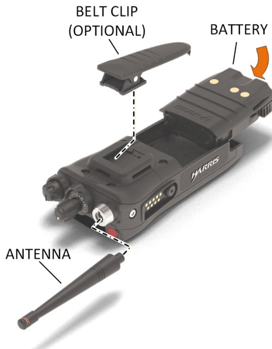
Figure 4-1: Radio Assembly
